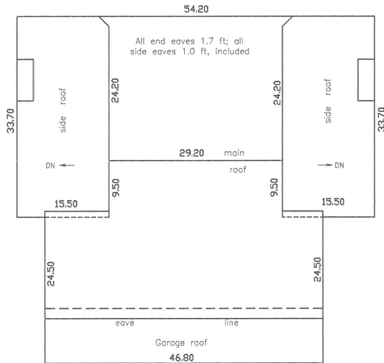
ROOF PLAN
