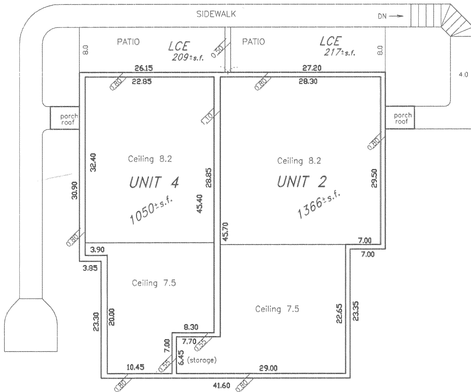
LOWER UNITS
