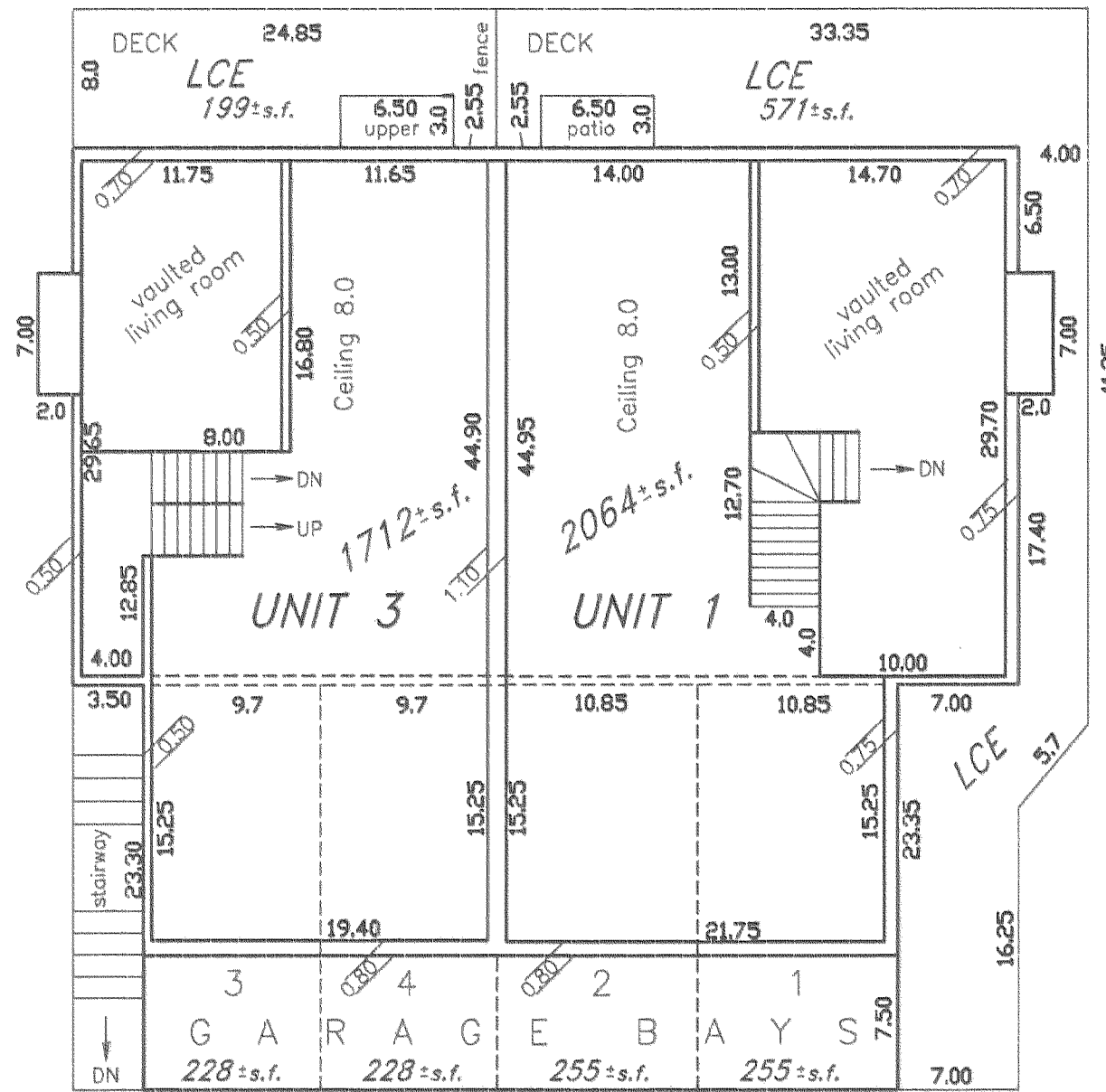
UPPER UNITS
