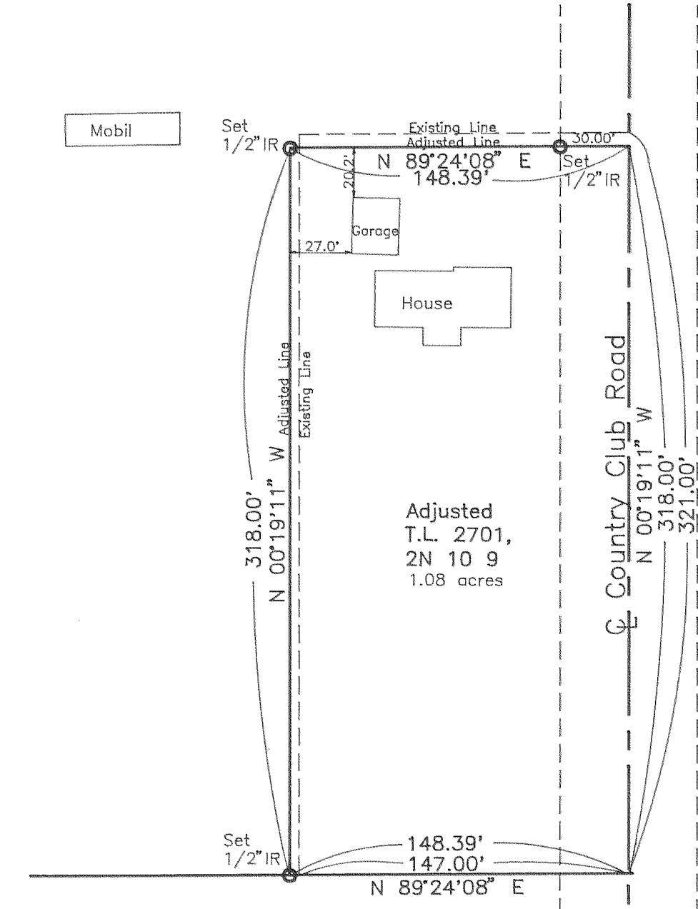
DETAIL 1" = 60'
