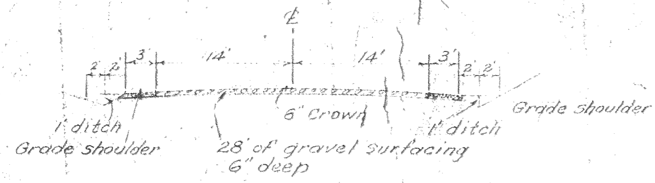
Roads Typical Section Scale: 1"=10'
