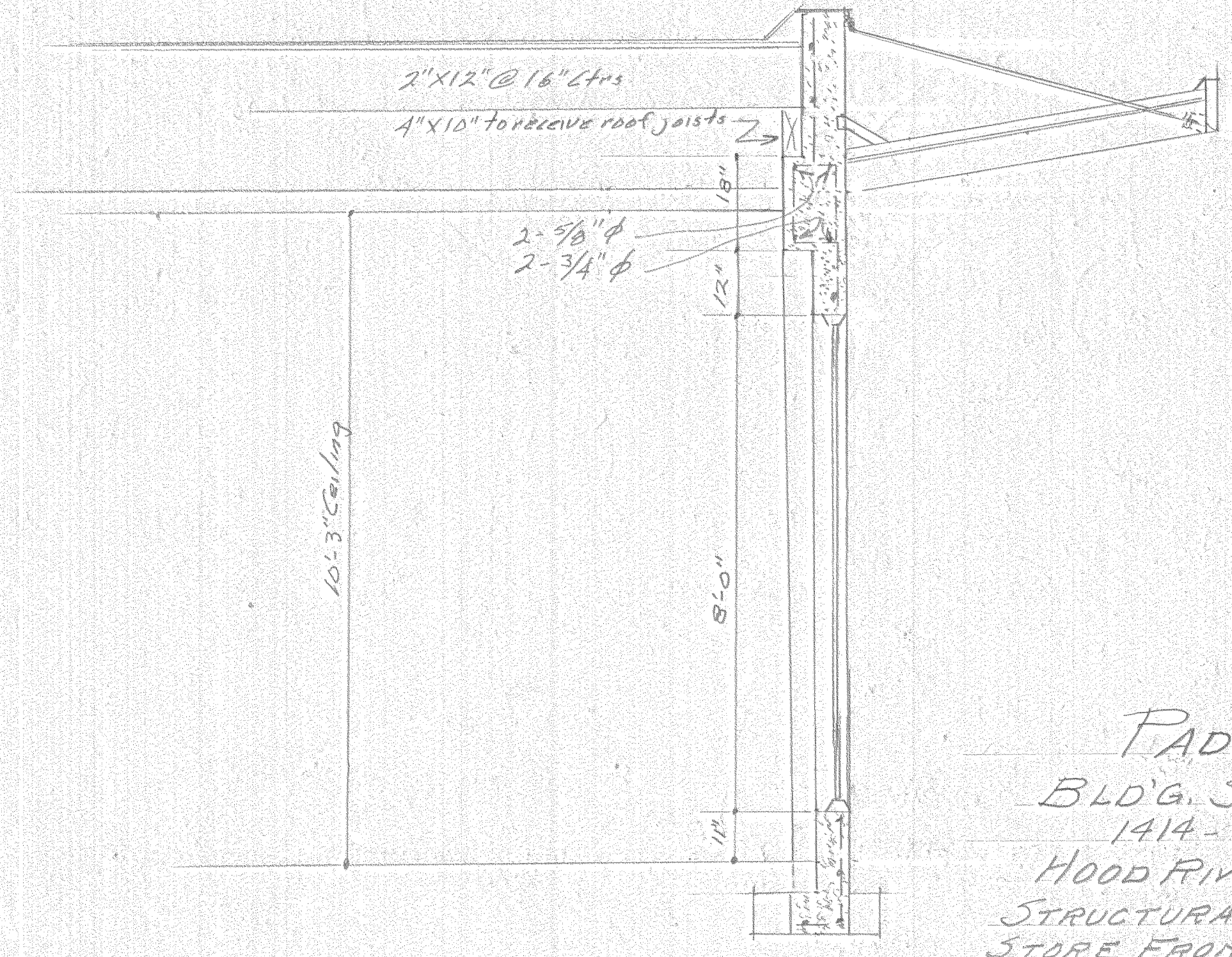
SEC. B-B Scale - \frac{1}{2} = 1'-0''
