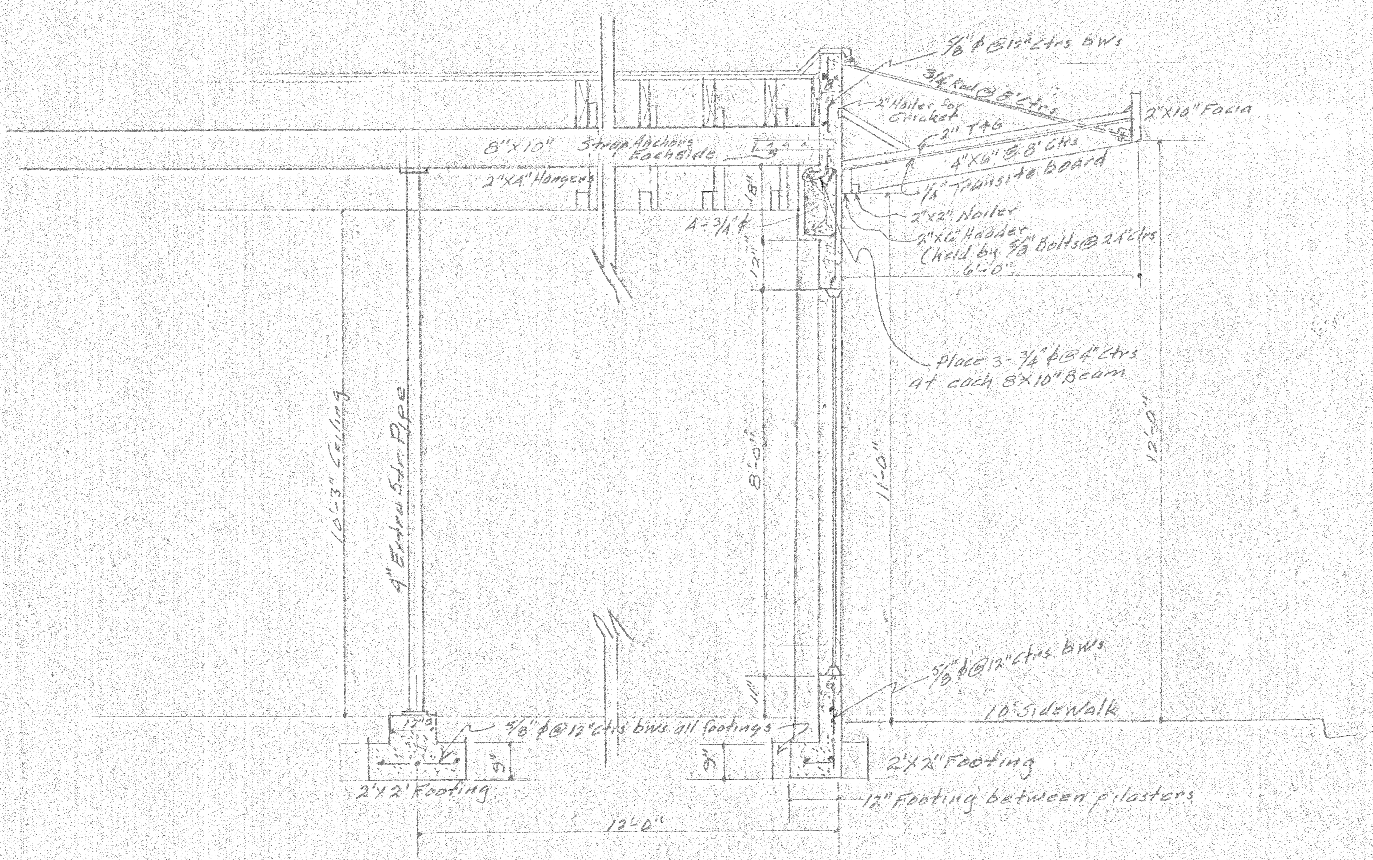
SEC. A-A Scale - \frac{1}{2} = 1'-0''
