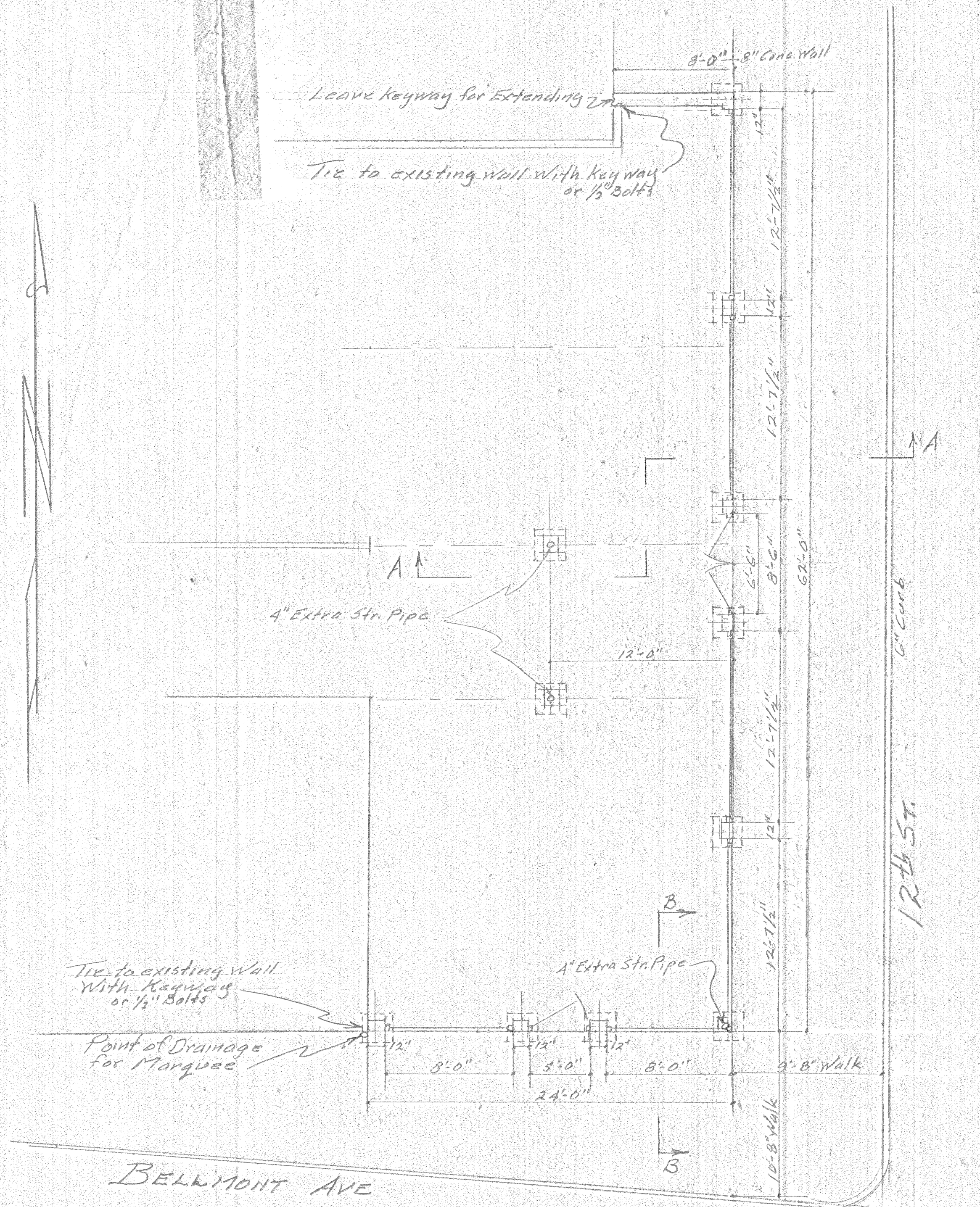
PLAN Scale \frac{3}{16} = 1'-0''
