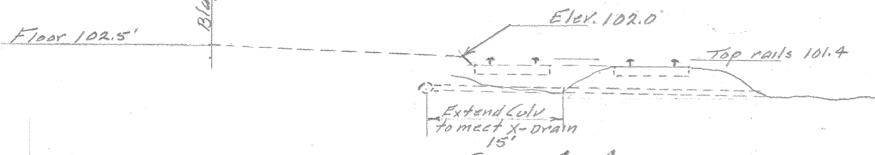
SEC A-A Scale 1"=10'
