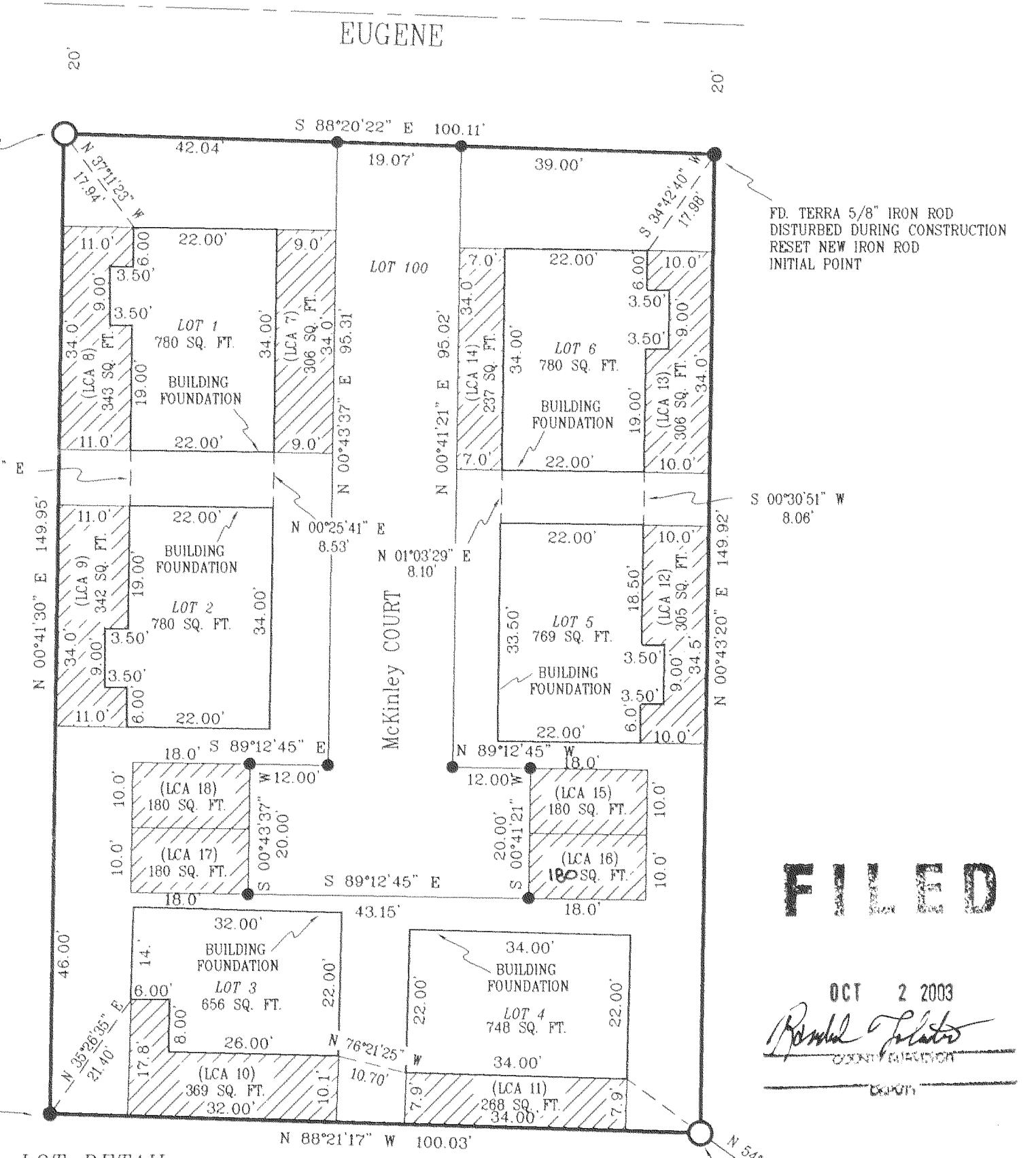
LOT DETAIL SCALE 1" = 20'
